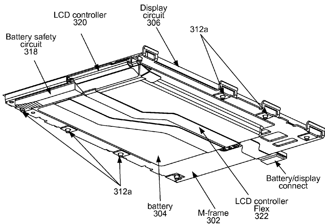
Fig. 2D M frame (assembled)
